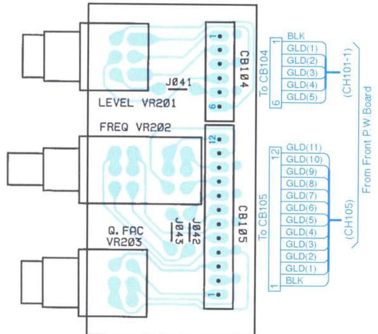
Volume(2) P.W.Board (Component Side View)
