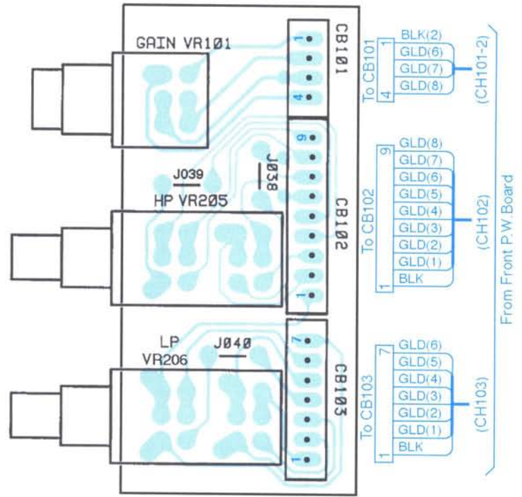
Volume(1) P.W.Board (Component Side View)
