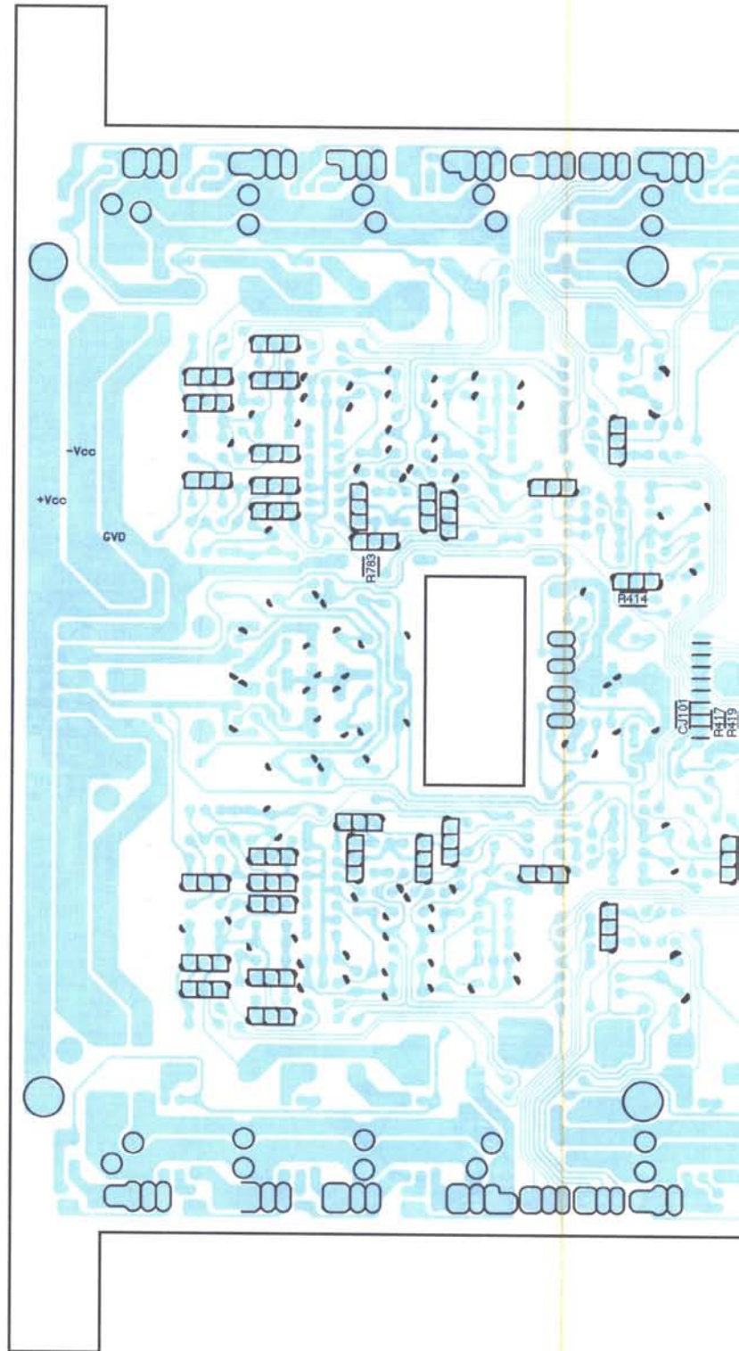
Front P.W.Board (Foil S
