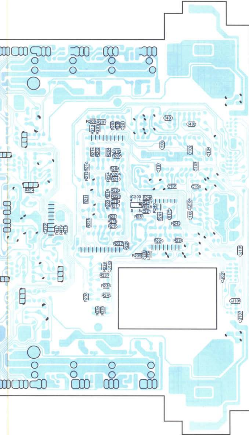
Board (Foil Side View)
